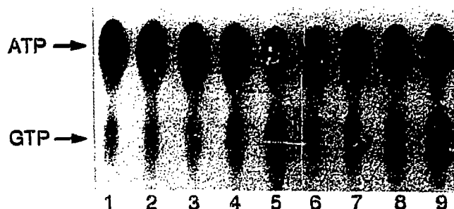
Fig. 4. Stimulation of NDP kinase activity by phospholipids or CHAPS. NDP kinase (5 ng/ml; 50 pM) was incubated with 0.5 \mu M [ \gamma - ^{32}P ]ATP and 1 \mu M GDP at 30°C for 6 min in 25 mM Na-HEPES buffer (pH 7.4) containing 2 mM MgCl_2 , 0.1 mM EDTA, 1 mM DTT, and the various concentrations of phospholipid (azolectin) or CHAPS. The reaction mixtures, after being diluted with a stop solution, were spotted on a thin layer chromatography plate and then developed as described in section 2.2. The radioactivity of ^{32}P in the fractions of [ \gamma - ^{32}P ]GTP and [ \gamma - ^{32}P ]ATP was visualized by autoradiography. (Lane 1) no additives; (lanes 2-5) 1, 10, 50, 300 \mu g/ml of azolectin, respectively; (lanes 6-9) 0.001, 0.003, 0.01, 0.1% CHAPS, respectively.
